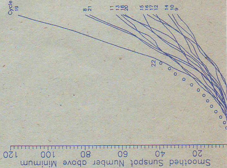
Rise of Solar Cycle 22 compared to previous Cycles
